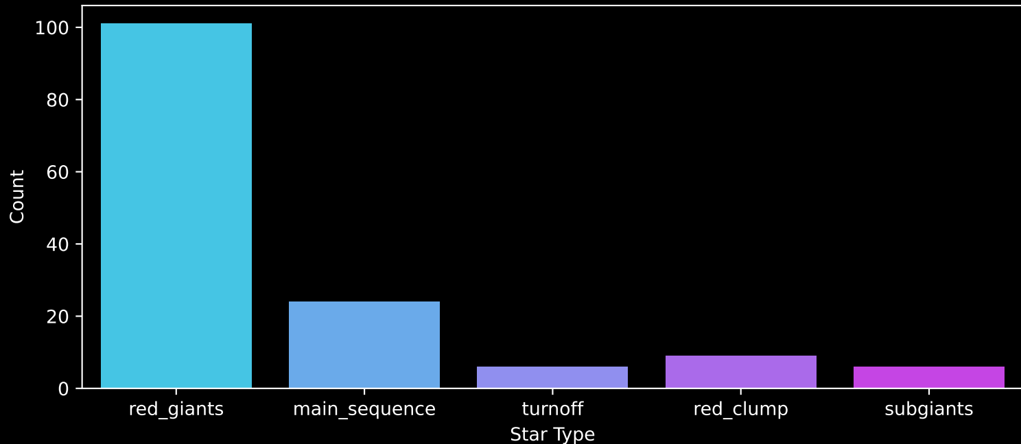
APOGEE DR17 Field: [135-12] Count plot of Star Type
