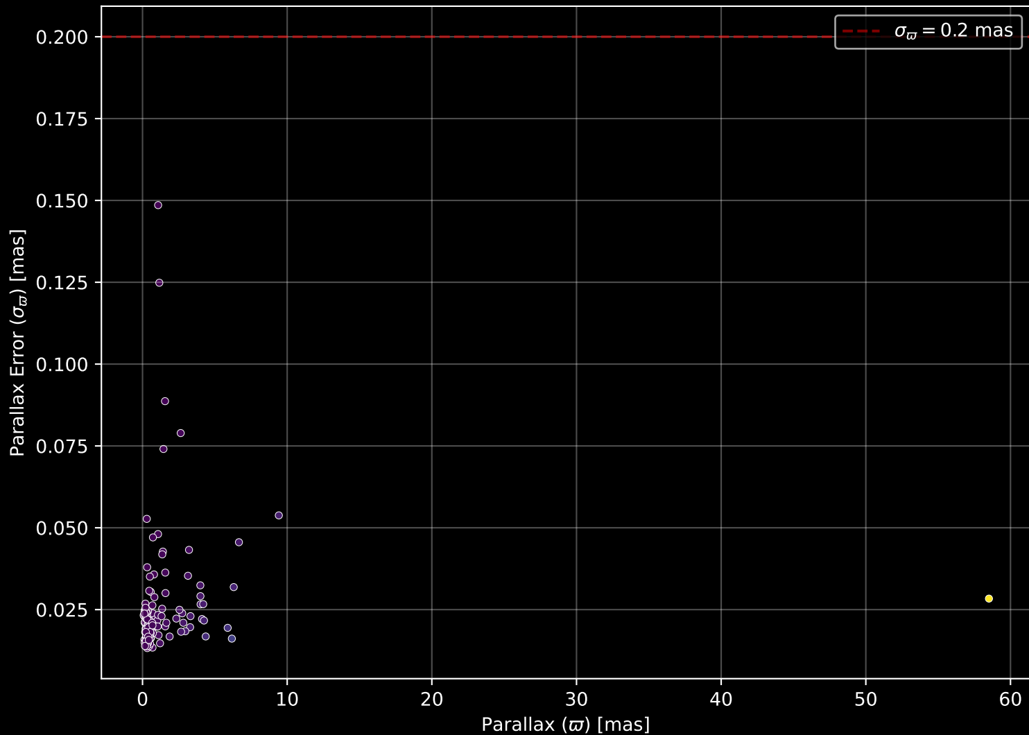
APOGEE DR17 Field: [135-12] Parallax Quality (n= 146)
