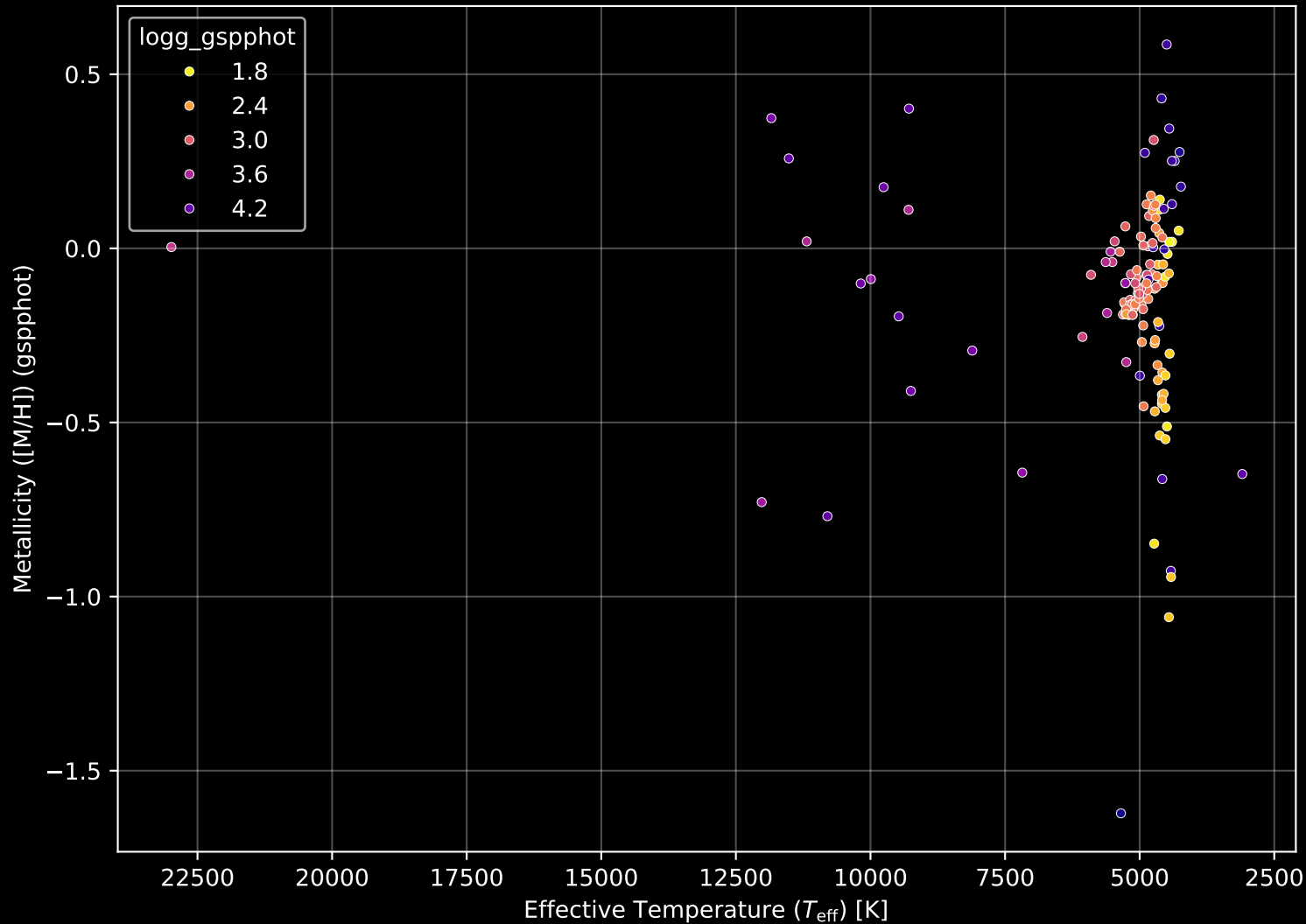
APOGEE DR17 Field: [135-12] Stellar Population Parameters (n= 146)
