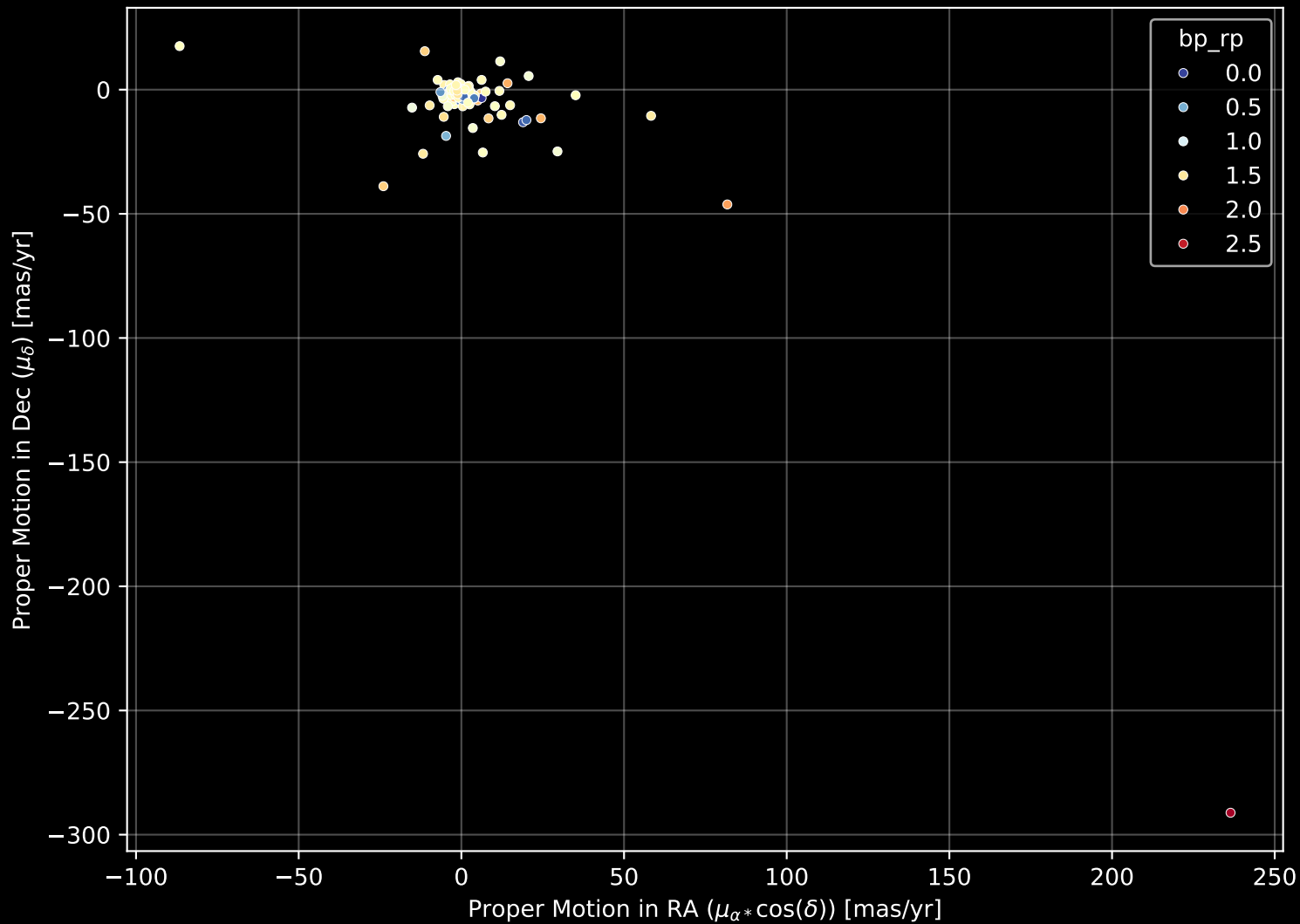
APOGEE DR17 Field: [135-12] Proper Motion Diagram (n= 146)
