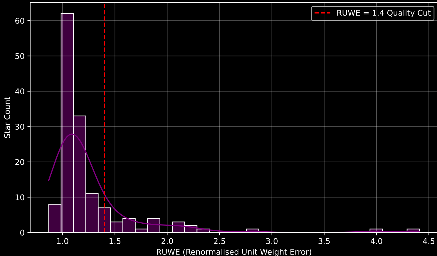
GAPOGEE DR17 Field [135-12] RUWE Distribution (n= 142)
