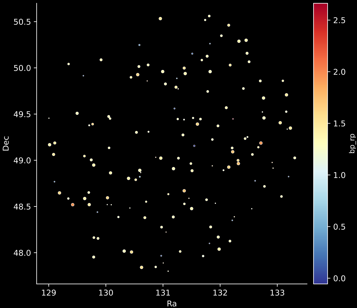
APOGEE DR17 Field: [135-12] Stars: 146
