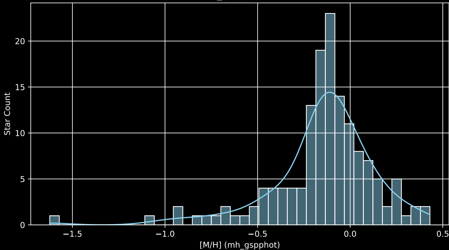
APOGEE DR17 Field: [135-12 [M/H] (mh_gspphot) (n= 145)
